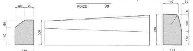
Raccord T3/A2 - RACCORD GAUCHE
