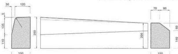
Raccord T2/A2 - RACCORD DROIT
