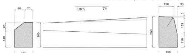
Raccord T2/A2 - RACCORD GAUCHE
