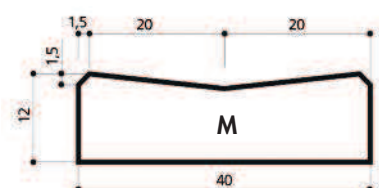
CC1
