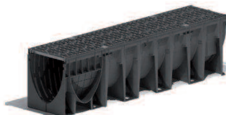
X200C, 1m, grille passerelle fonte
